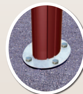
Quatro post on base plates
